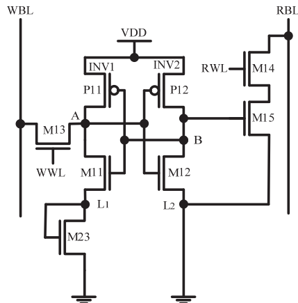
Figure 5. The simplified circuit diagram during the write operation.
