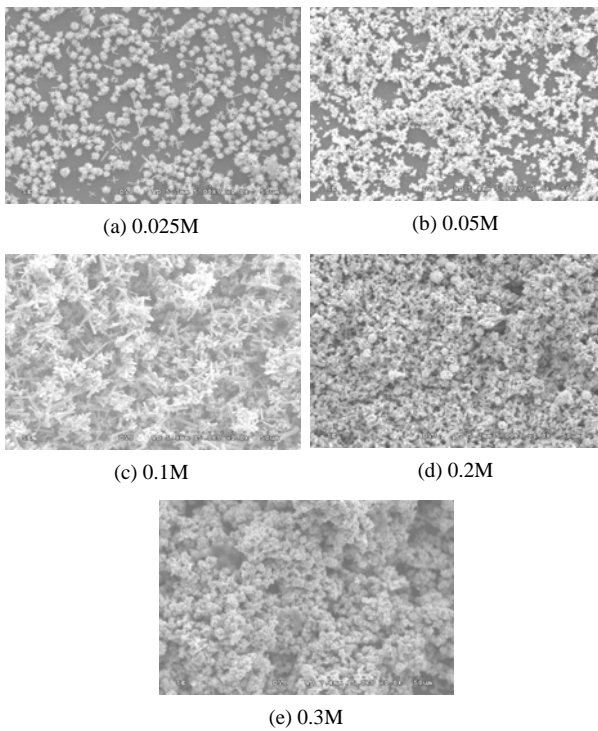
Fig. 1. The top-view SEM images of ZnO nanorods prepared by various concentrations of \text{Zn}(\text{NO}_3)_2 \cdot 6\text{H}_2\text{O} + \text{C}_6\text{H}_{12}\text{N}_4 . The magnification factor is 1 \times 10^3 .
