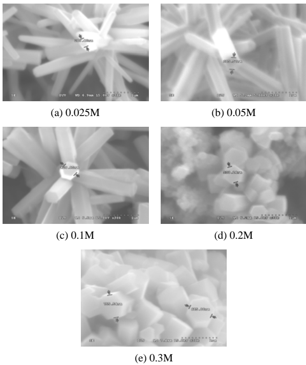
Fig. 2. The enlarged top-view SEM images of ZnO nanorods prepared by various concentrations of \text{Zn}(\text{NO}_3)_2 \cdot 6\text{H}_2\text{O} + \text{C}_6\text{H}_{12}\text{N}_4 . The magnification factor is 3 \times 10^4 .
