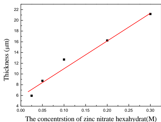
Fig. 4. Film thickness of ZnO nanorods prepared by various concentrations of \text{Zn}(\text{NO}_3)_2 \cdot 6\text{H}_2\text{O} + \text{C}_6\text{H}_{12}\text{N}_4 .
