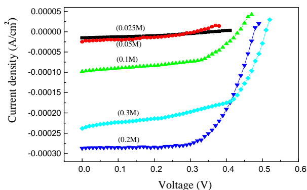
Fig. 6. J - V characteristics of the DSSCs using ZnO nanorods prepared by various concentrations of \text{Zn}(\text{NO}_3)_2 \cdot 6\text{H}_2\text{O} + \text{C}_6\text{H}_{12}\text{N}_4 as the working electrode.
