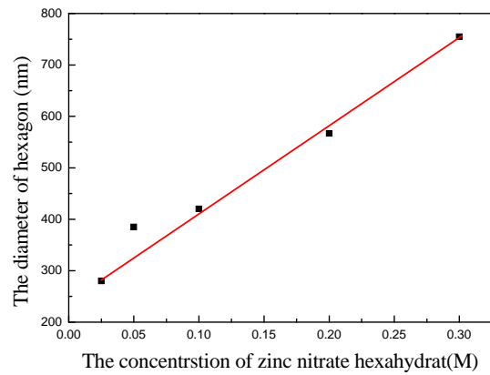
Fig. 3. Average diameter of ZnO nanorods prepared by various concentrations of \text{Zn}(\text{NO}_3)_2 \cdot 6\text{H}_2\text{O} + \text{C}_6\text{H}_{12}\text{N}_4 .
