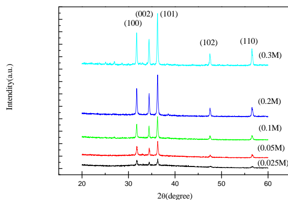
Fig. 5. XRD spectra for the ZnO nanorods prepared by various concentrations of \text{Zn}(\text{NO}_3)_2 \cdot 6\text{H}_2\text{O} + \text{C}_6\text{H}_{12}\text{N}_4 .
